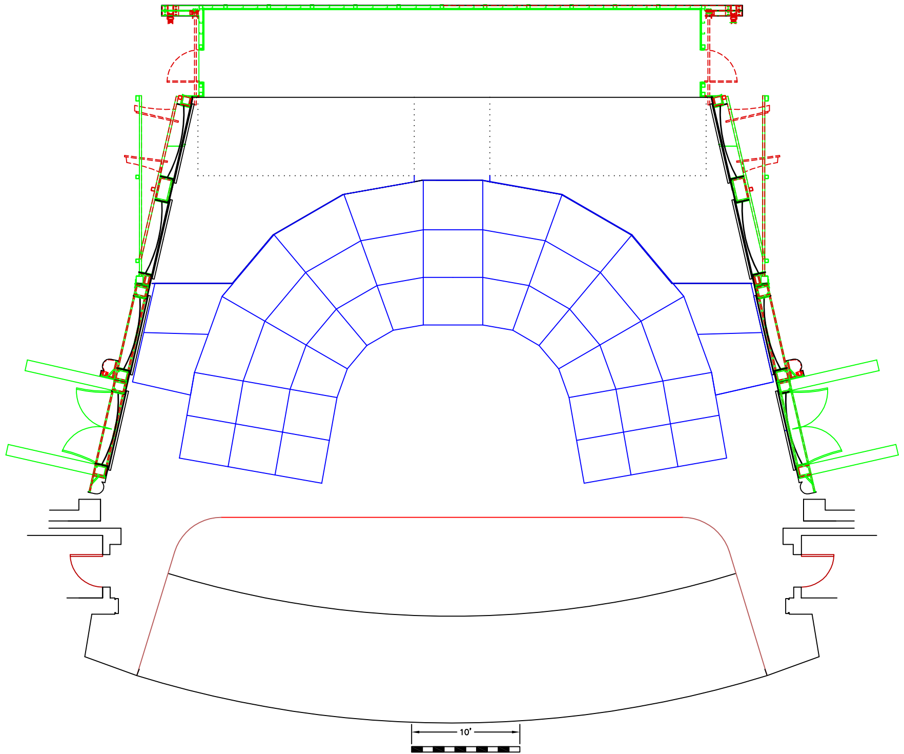
PLAN VIEW OF ORCHESTRA SHELL – LARGE
